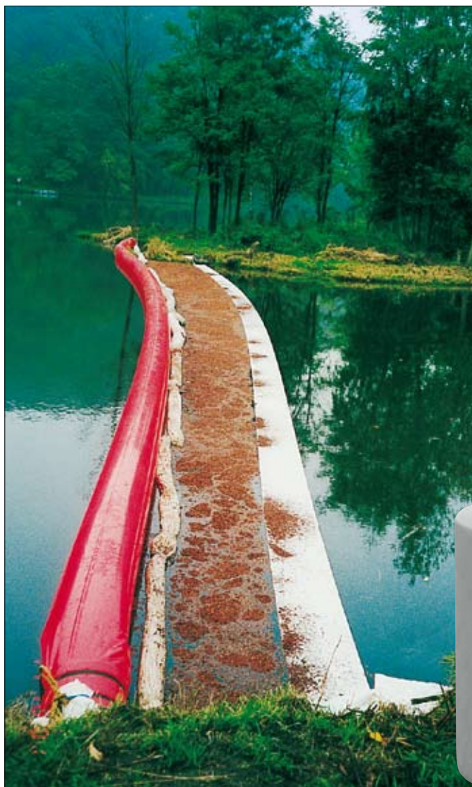
Absorption of the oil slick in front of the spill containment boom with the help of the absorptive mat and loose sorbent
