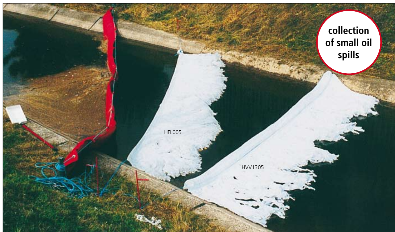
Final treatment of water surface with the help of hydrophobic pollution catcher HFL005 and hydrophobic absorbent boom with fibres HVV1305
